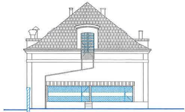
FACADE SUD
